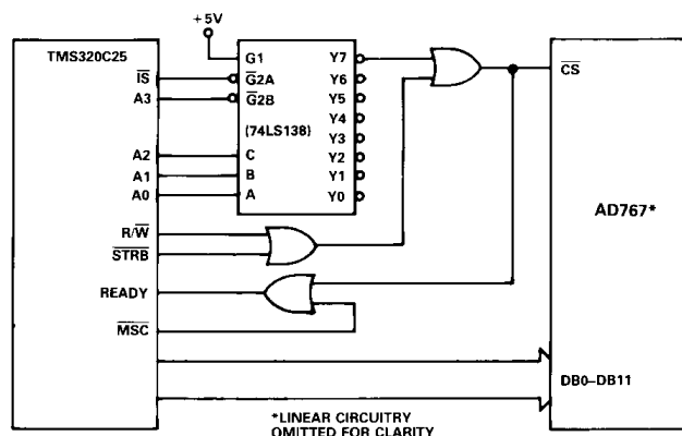
Figure 11. TMS320C25 – AD767 Interface
